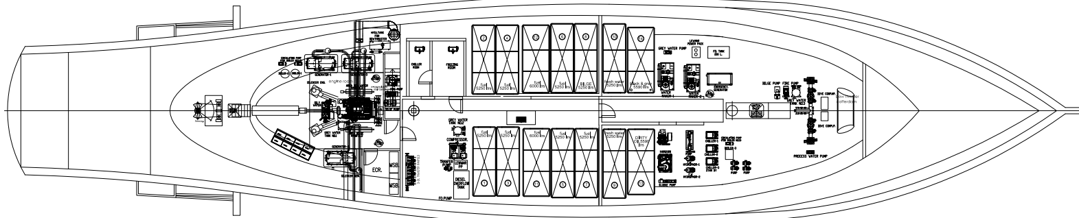
tank deck
