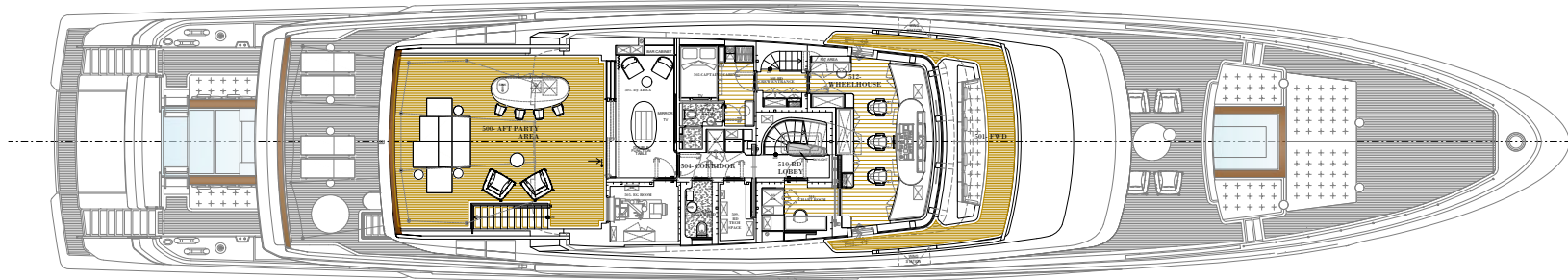
BRIDGE DECK
